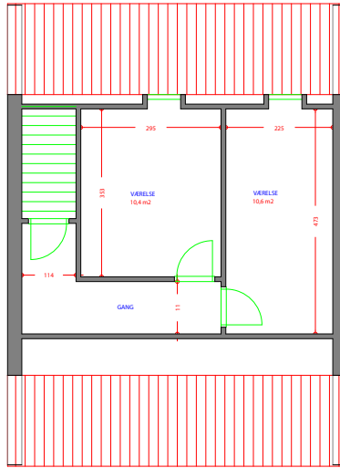
AFDELING 1 TYPE 44 4 RUMS 94M2 1.SAL
