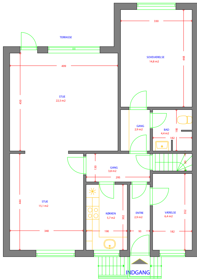
AFDELING 1 TYPE 43 4 RUMS 88M2 STUEPLAN
