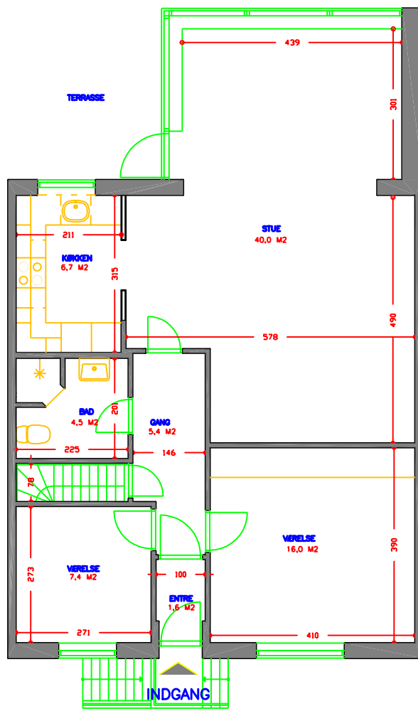
AFDELING 1 TYPE 37 3 RUMS 98 M2 STUEPLAN
