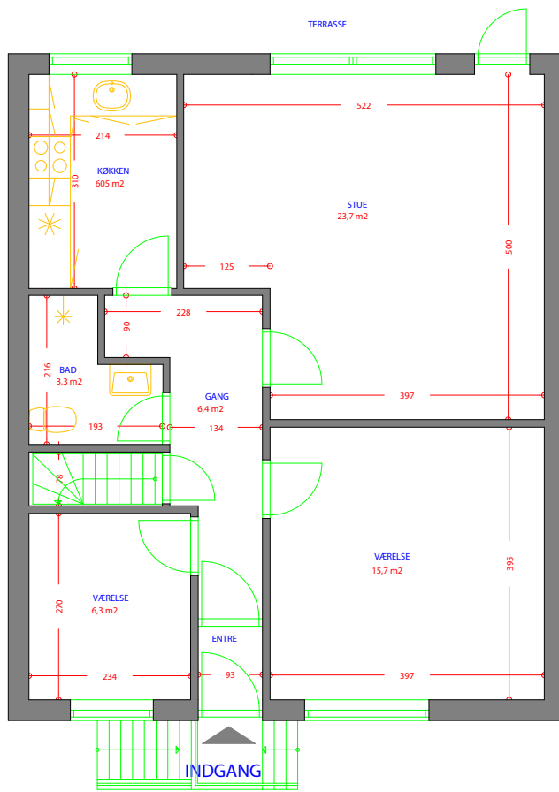
AFDELING 1 TYPE 33 3 RUMS 80M2 STUEPLAN
