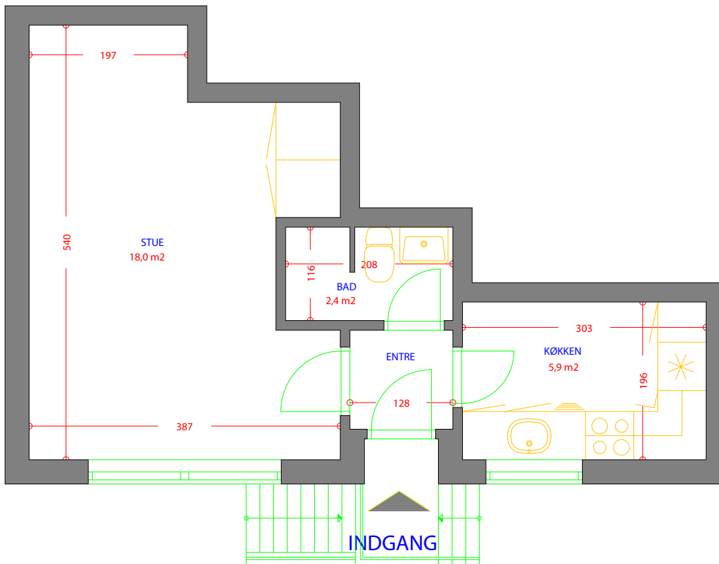
AFDELING 1 TYPE 11 1 RUMS 39M2 STUEPLAN
